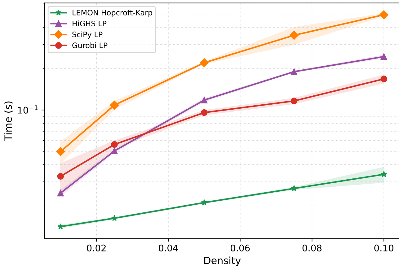
Runtime vs density (n=1024)
