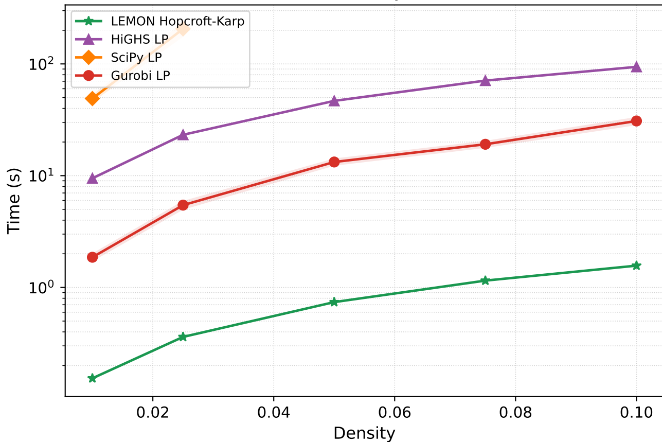
Runtime vs density (n=8192)
