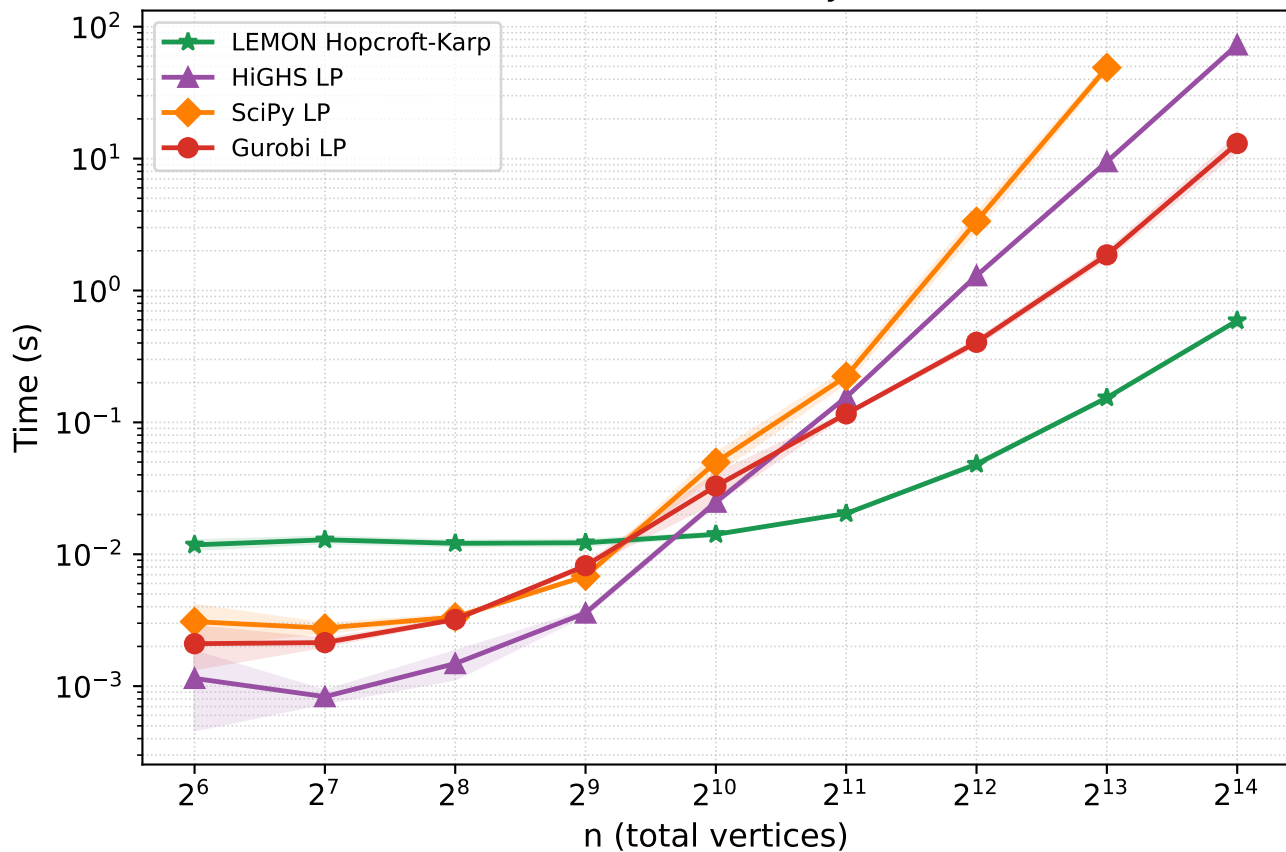
Runtime vs n (density=0.01)
