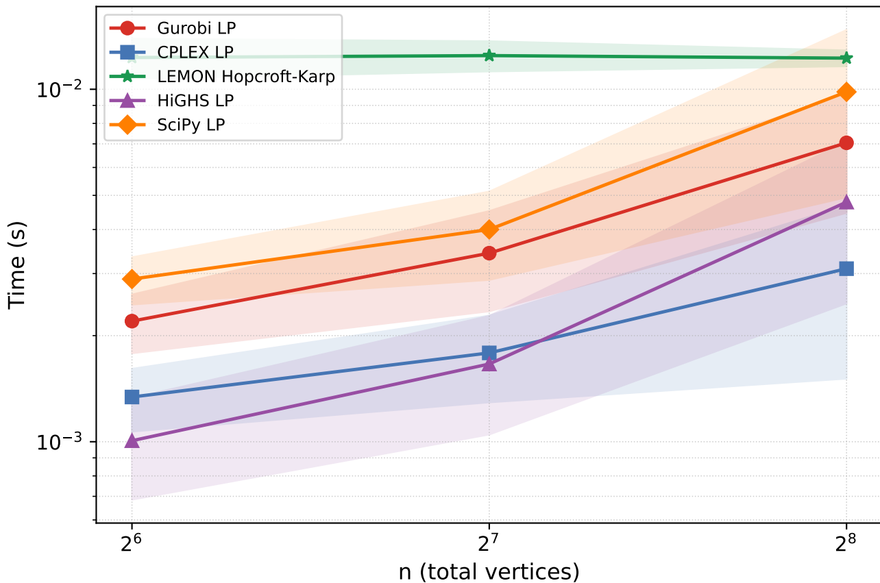
Small instances with CPLEX (n ≤ 256)
