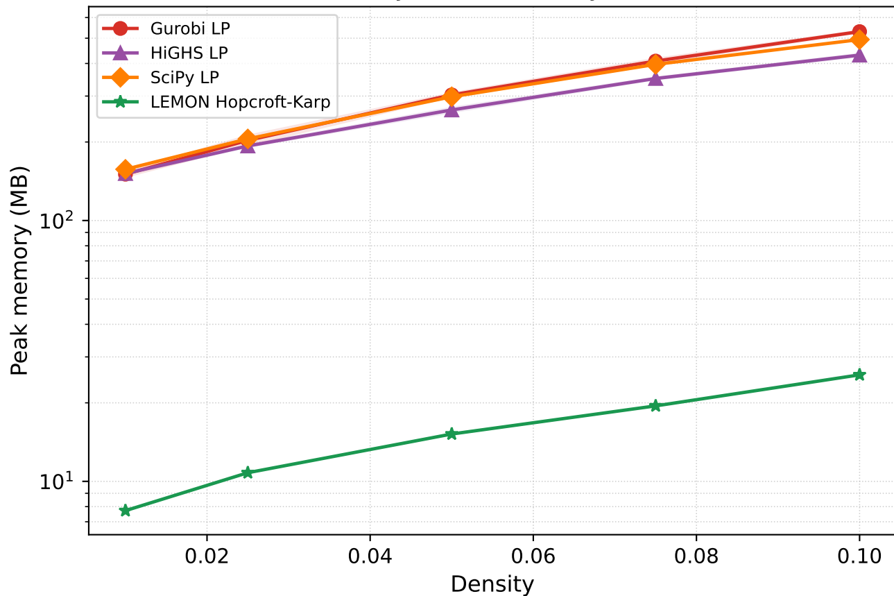
Peak memory (MB) vs density ( n = 4096 )
