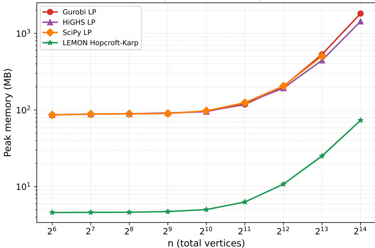
Peak memory (MB) vs n (density = 0.025)
