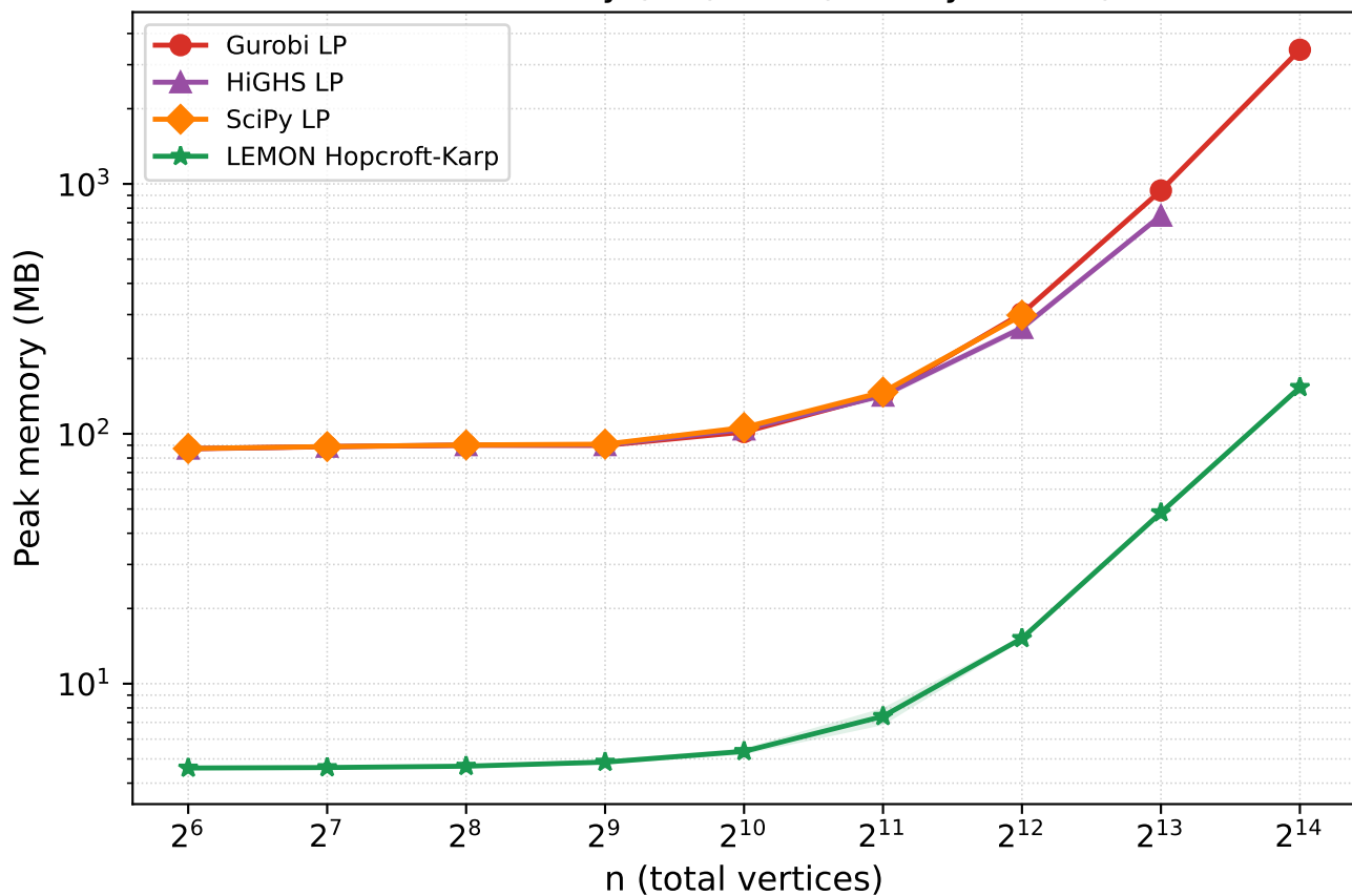
Peak memory (MB) vs n (density = 0.05)
