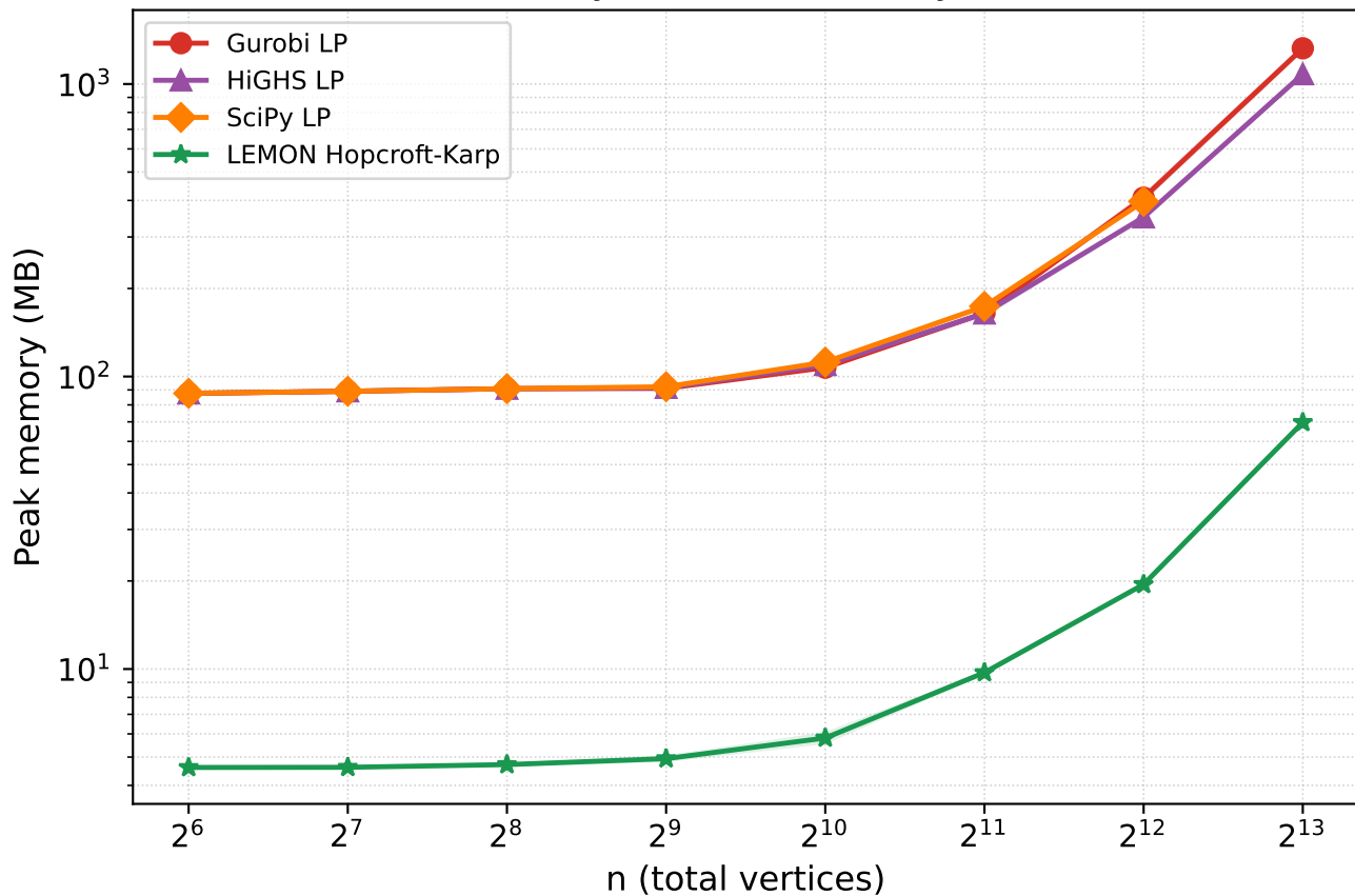
Peak memory (MB) vs n (density = 0.075)
