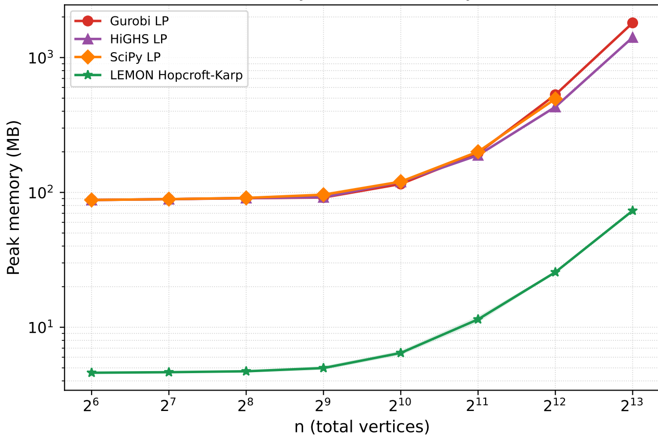
Peak memory (MB) vs n (density = 0.1)
