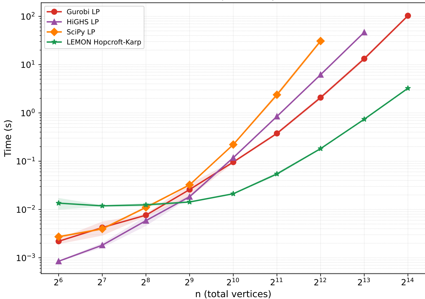
Solver landscape (density = 0.05)
