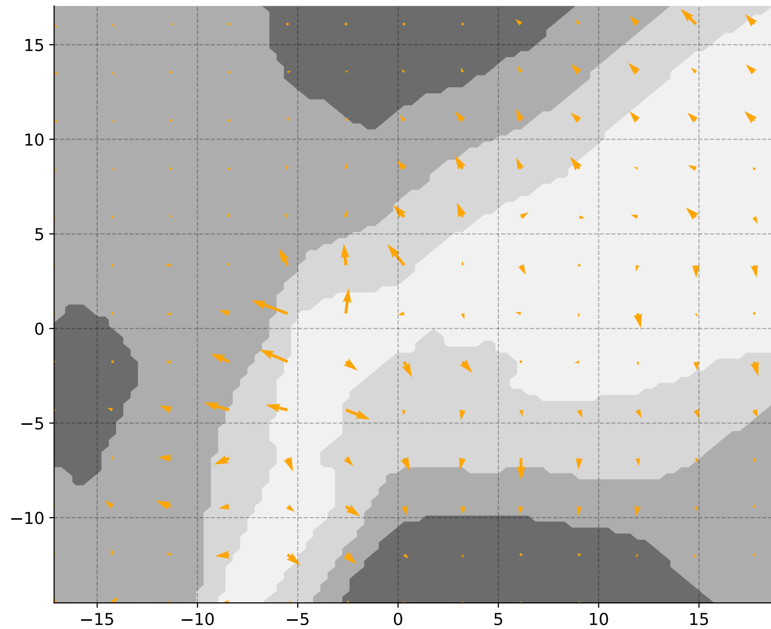
Gradient Field for Pixel 350 (Target: Class 3)
