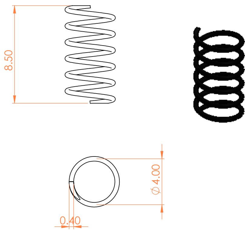
Part8_Spring
