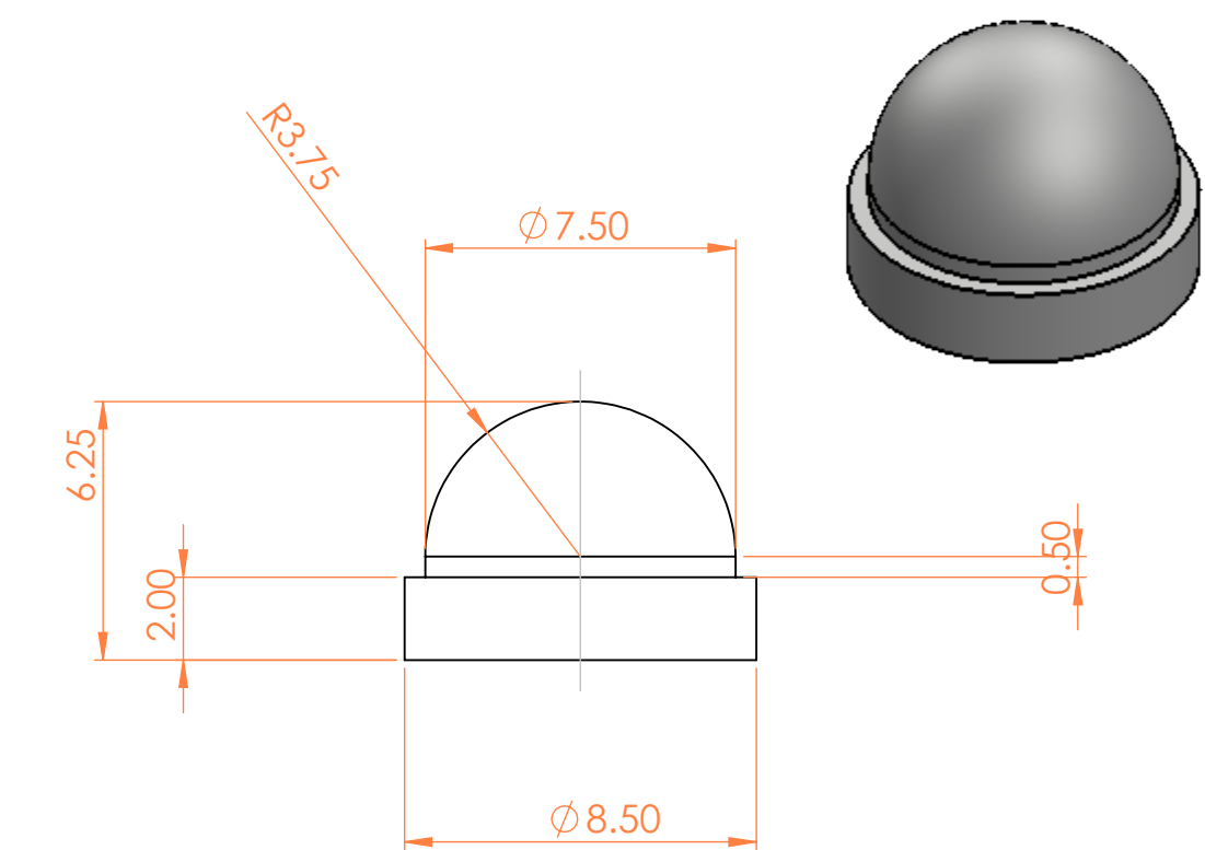
Part7_clampButton
