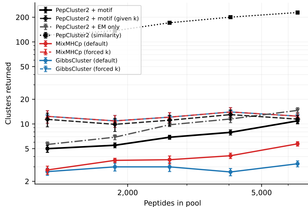
Granularity of the returned partition (independent test pools)
