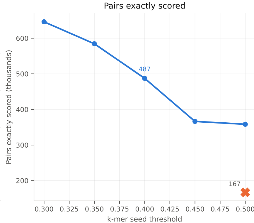
Redesigned terminal seed: sensitivity against cost (graph, coverage order, 5 datasets)
