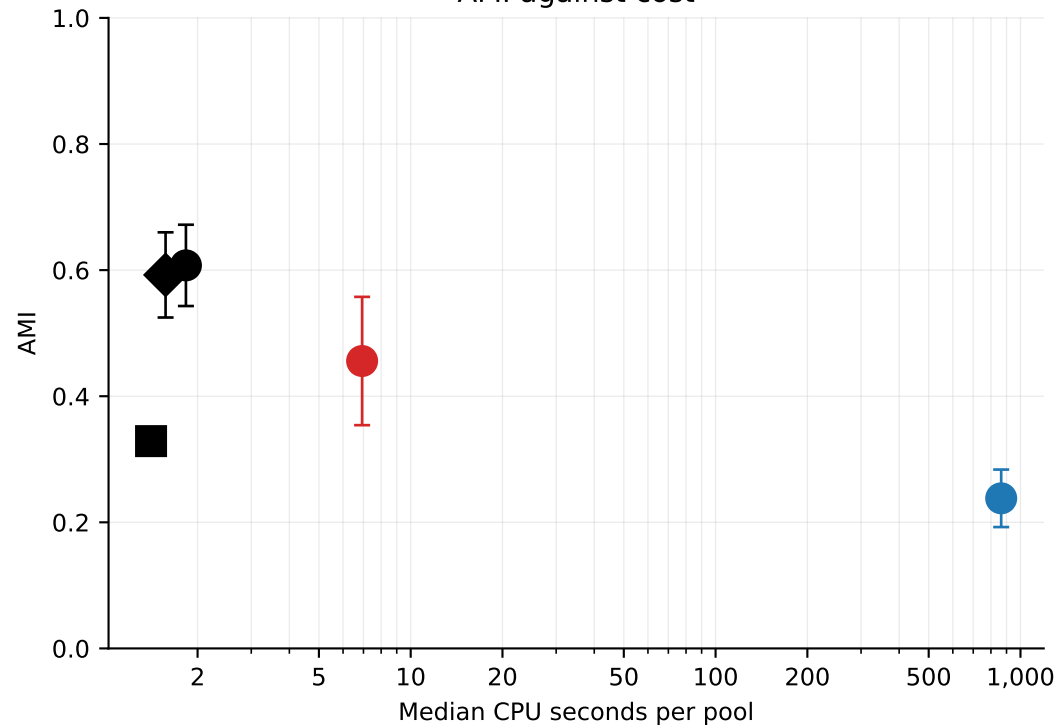
AMI against cost
