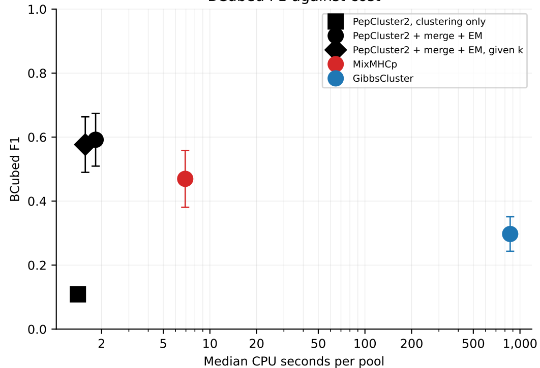
BCubed F1 against cost
