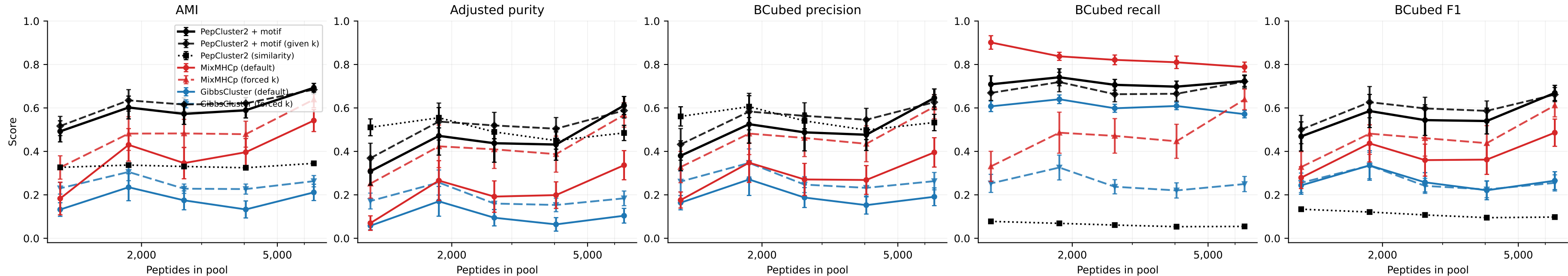
Performance against peptides in pool (independent test pools, mean \pm s.e.m.)
