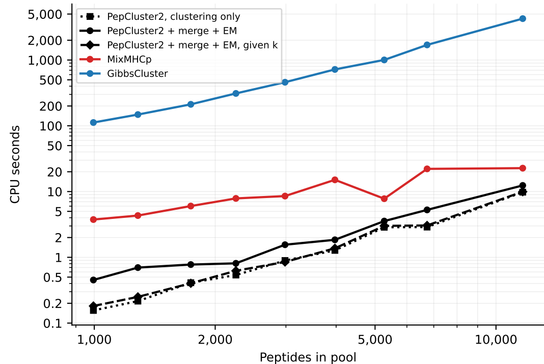
Cost against pool size (serial runs; PepCluster2 and MixMHCp single-threaded, GibbsCluster at -k 16)
