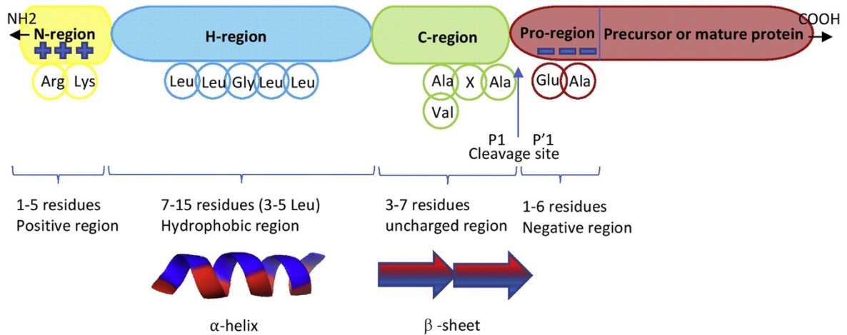
Figure 1. Schematic representation of a canonical SP. The SP contains an N-terminal region (1-5 residues), an H-region (7-15 residues), and a C-region (3-7 residues). Residues flanking the cleavage position are denoted P1 (upstream) and P'1 (downstream), and cleavage commonly occurs at motifs of the form A-X-A or V-X-A [3].
