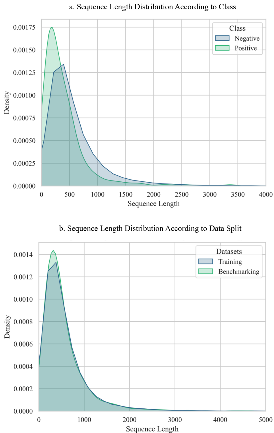
Figure S2. Sequence length distribution. (a) According to Class. In blue the negatives, in light green the positives. (b) According to Data Split. In blue the training set and in light green the benchmarking set.
