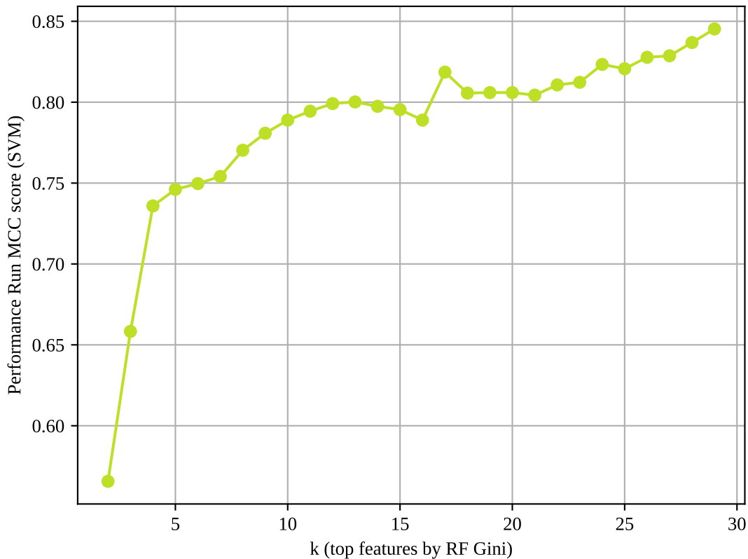
MCC vs. Number of Selected Features (Performance_Run)
