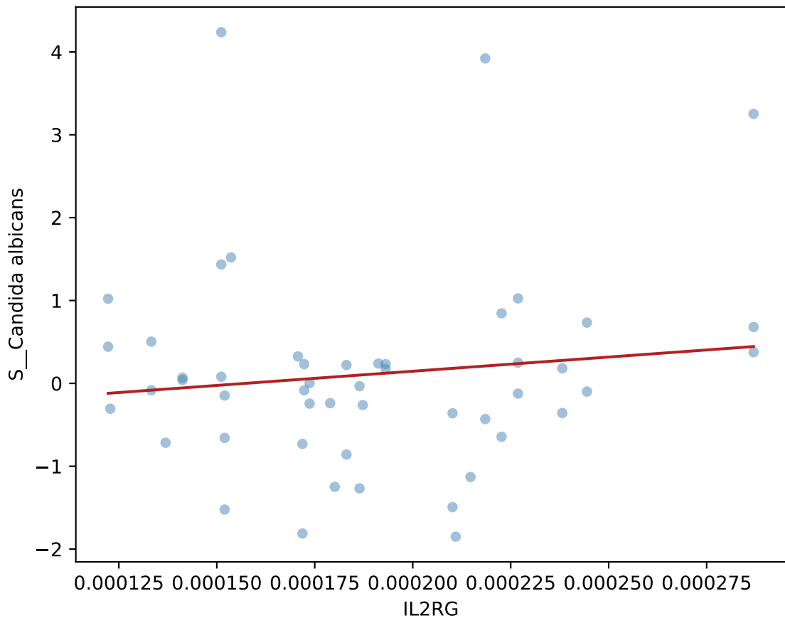
IL2RG vs. Candida albicans (+-4w, CD, n=50)
