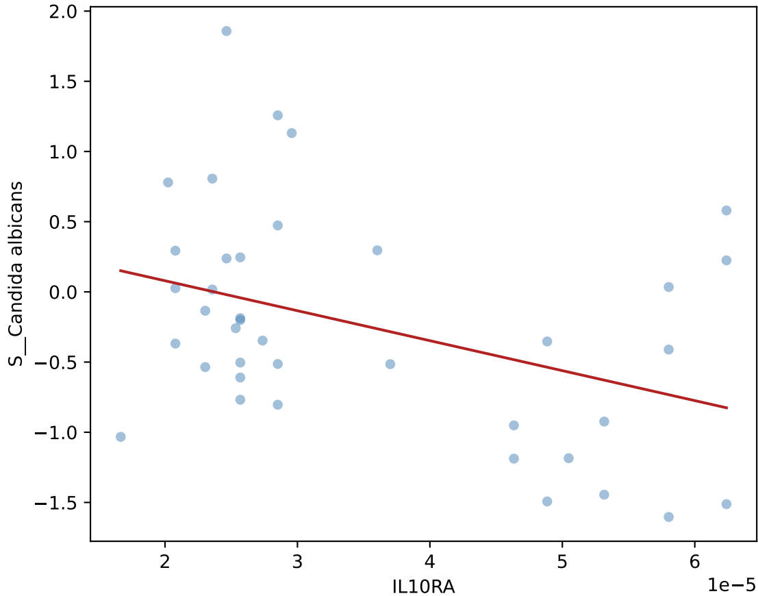
IL10RA vs. Candida albicans (+-4w, HD, n=39)
