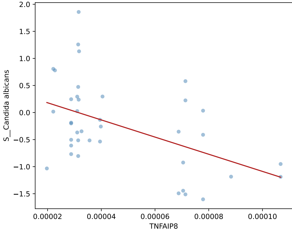
TNFAIP8 vs. Candida albicans (+-4w, HD, n=39)
