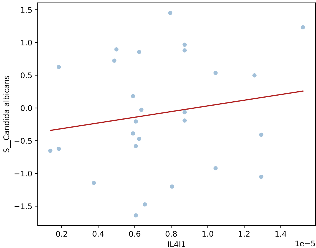
IL4I1 vs. Candida albicans (+4w, UC, n=27)
