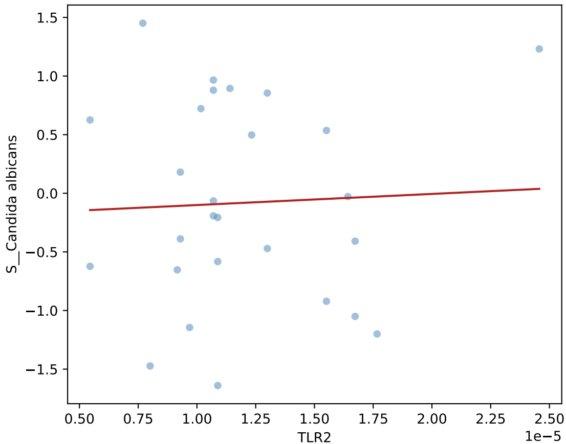
TLR2 vs. Candida albicans (+-4w, UC, n=27)
