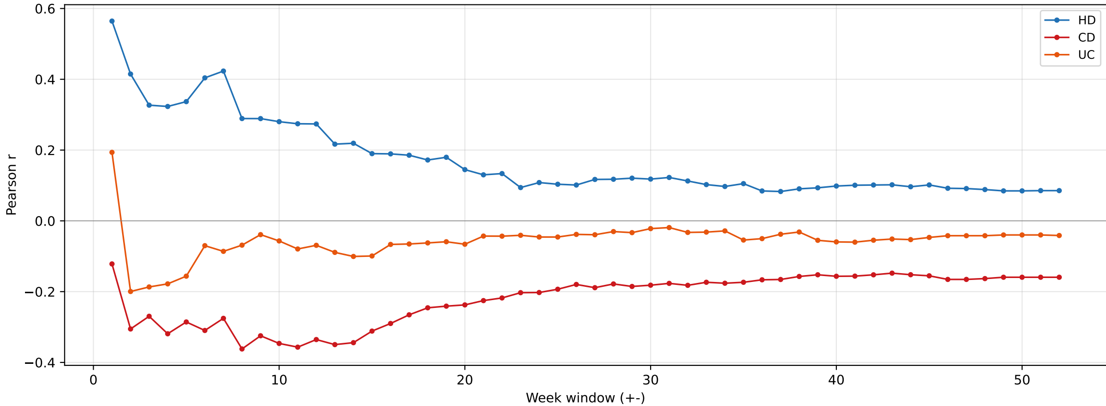
BTNL3 - Candida albicans correlation coefficient vs. week window
