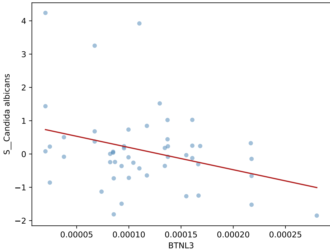
BTNL3 vs. Candida albicans (CD, +4w, n=50, r=-0.319 , p=2.39\text{e-}02 )
