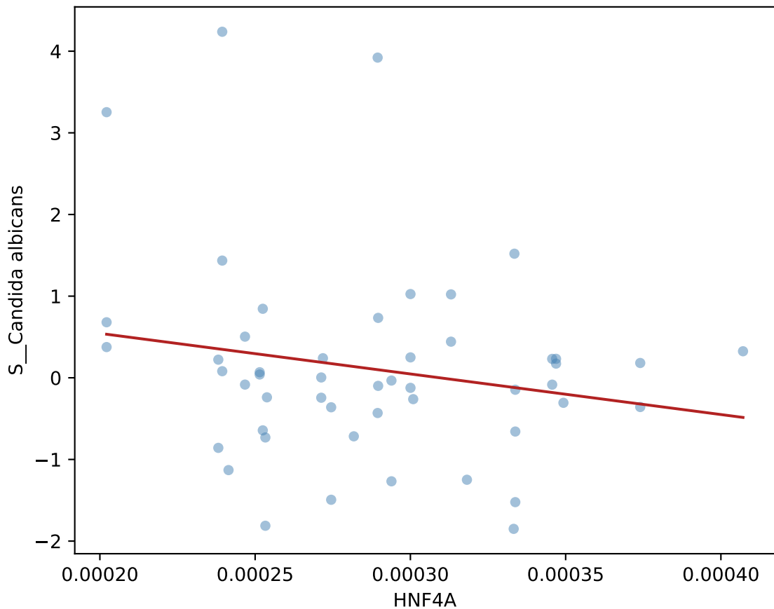
HNF4A vs. Candida albicans (+-4w, CD, n=50)
