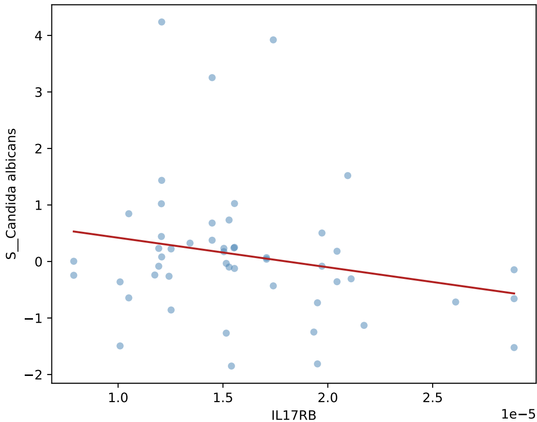
IL17RB vs. Candida albicans (+-4w, CD, n=50)
