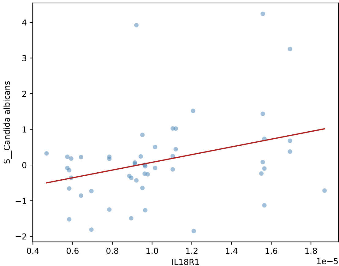
IL18R1 vs. Candida albicans (+-4w, CD, n=50)
