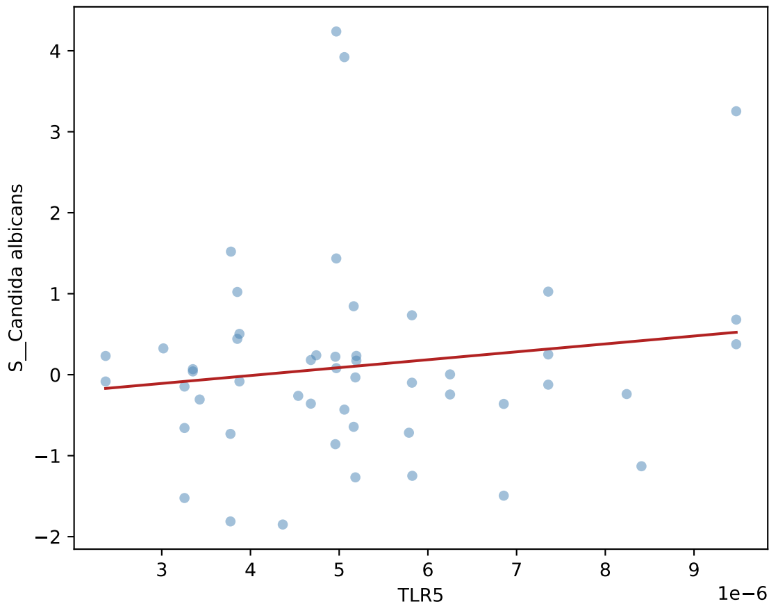
TLR5 vs. Candida albicans (+4w, CD, n=50)
