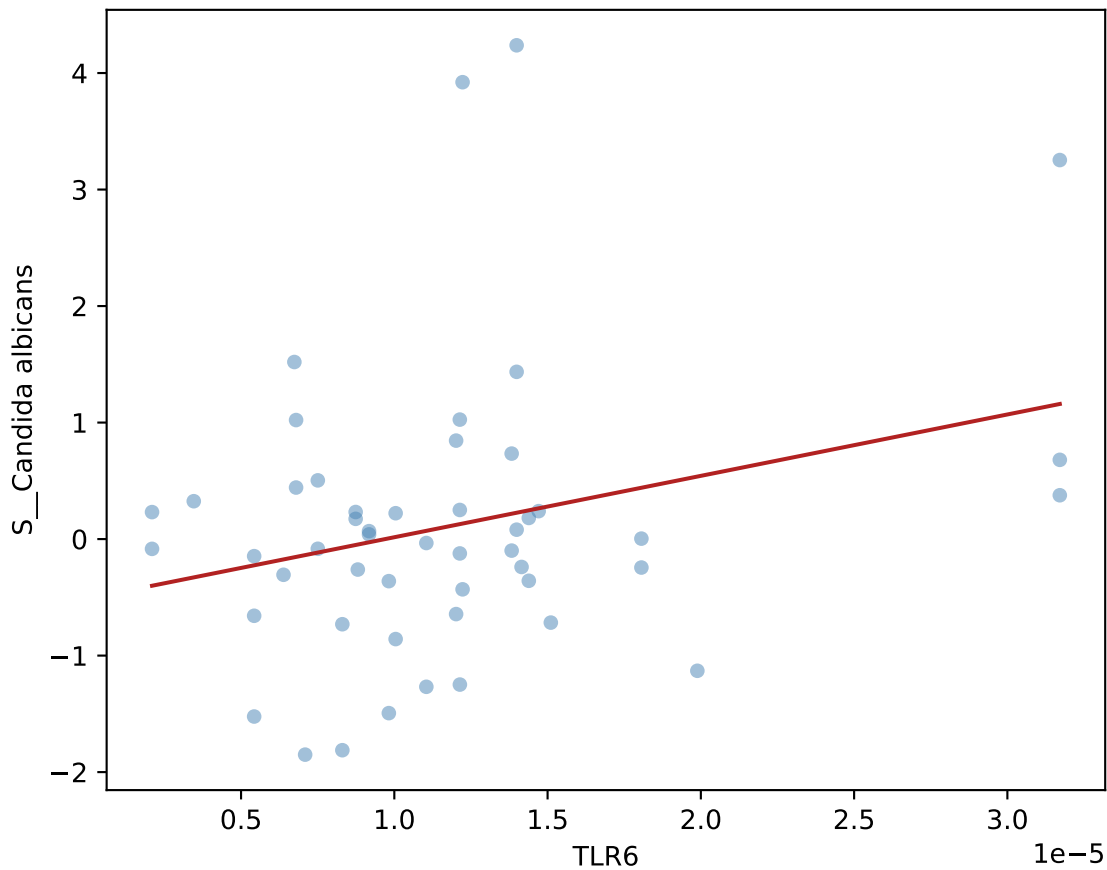
TLR6 vs. Candida albicans (+-4w, CD, n=50)
