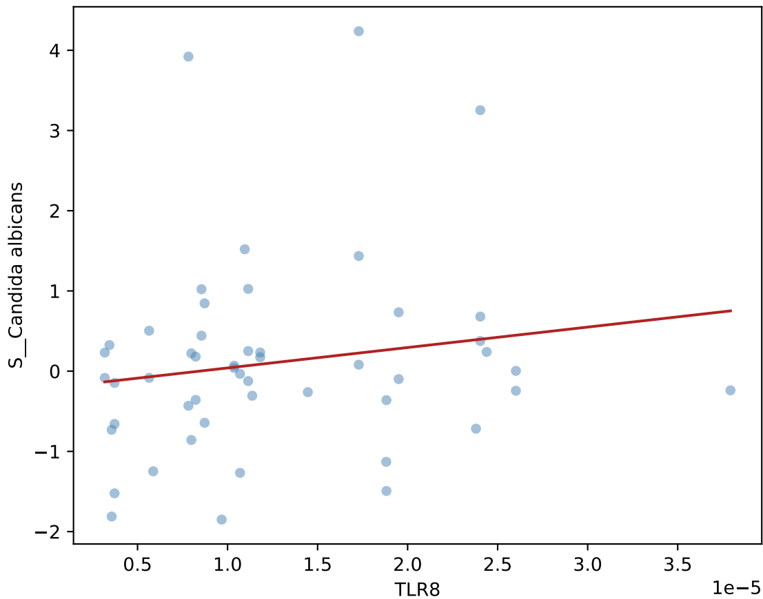
TLR8 vs. Candida albicans (+4w, CD, n=50)
