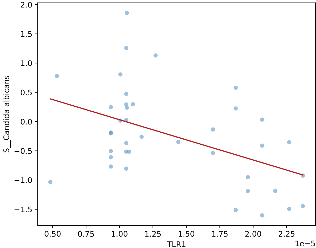
TLR1 vs. Candida albicans (+-4w, HD, n=39)
