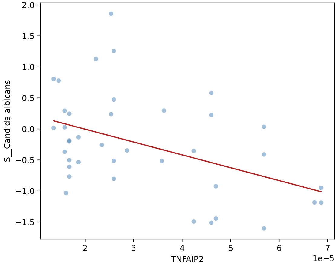
TNFAIP2 vs. Candida albicans (+-4w, HD, n=39)
