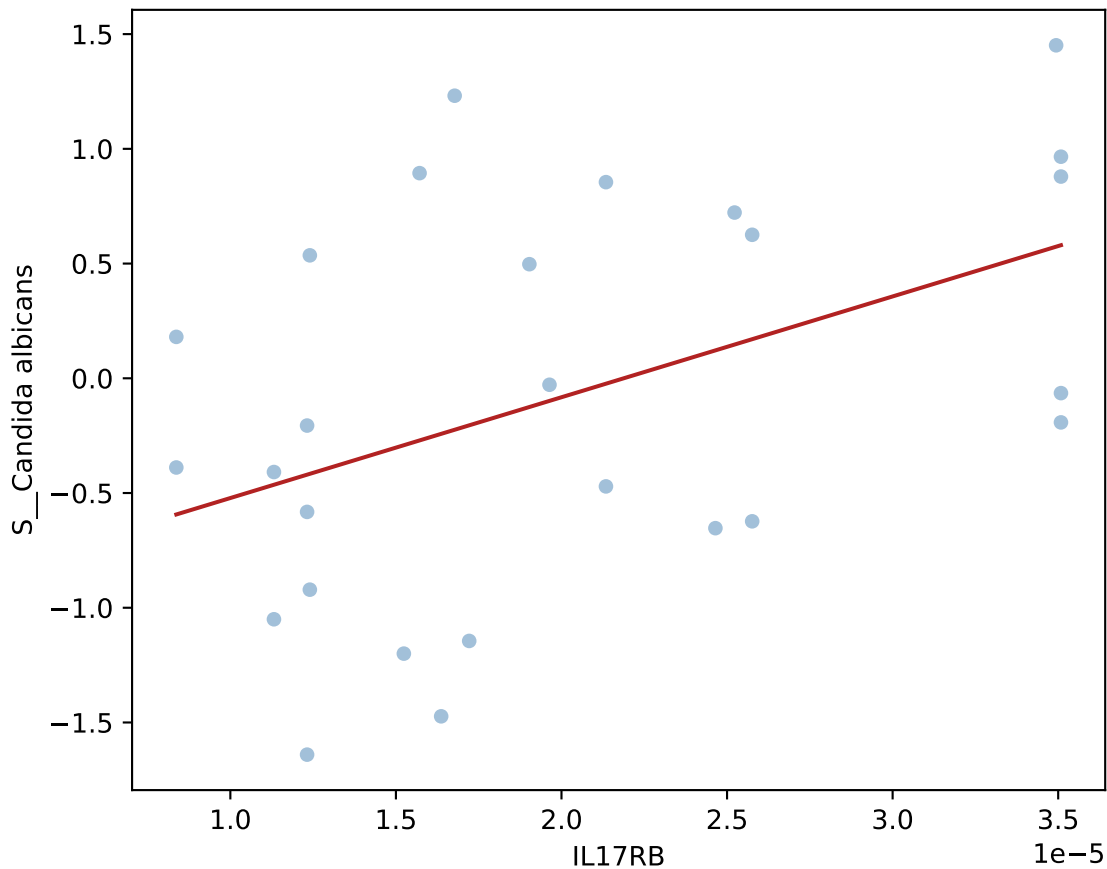
IL17RB vs. Candida albicans (+4w, UC, n=27)
