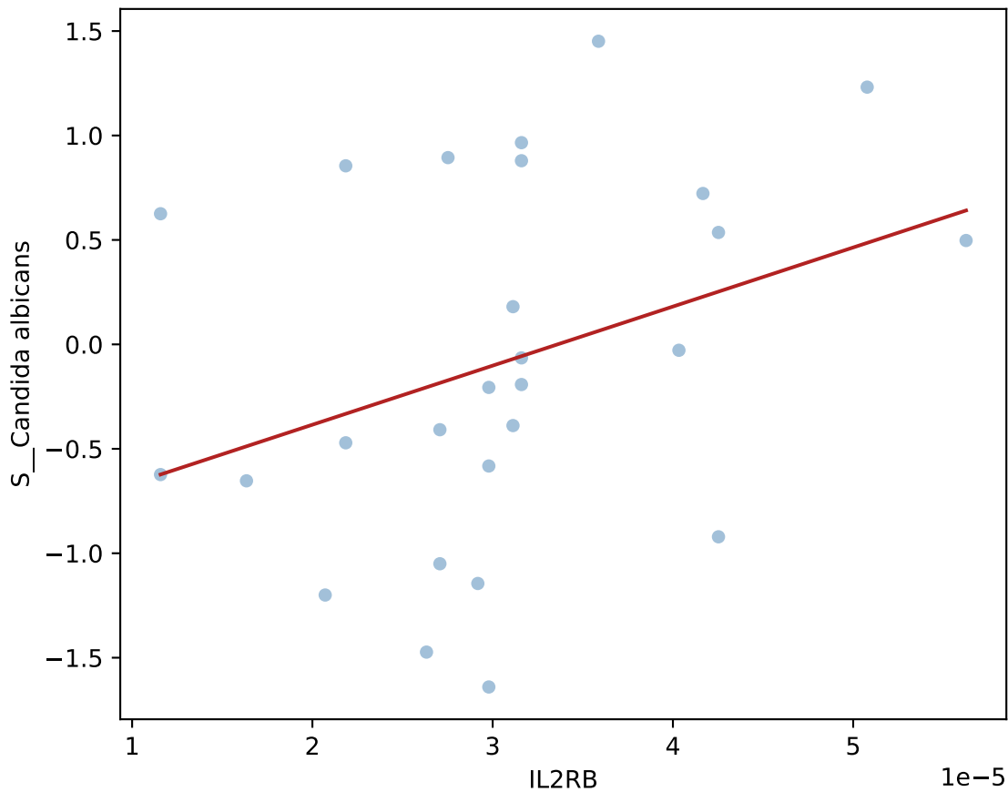
IL2RB vs. Candida albicans (+-4w, UC, n=27)
