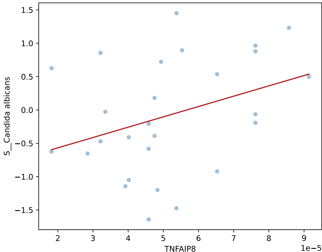
TNFAIP8 vs. Candida albicans (+-4w, UC, n=27)
