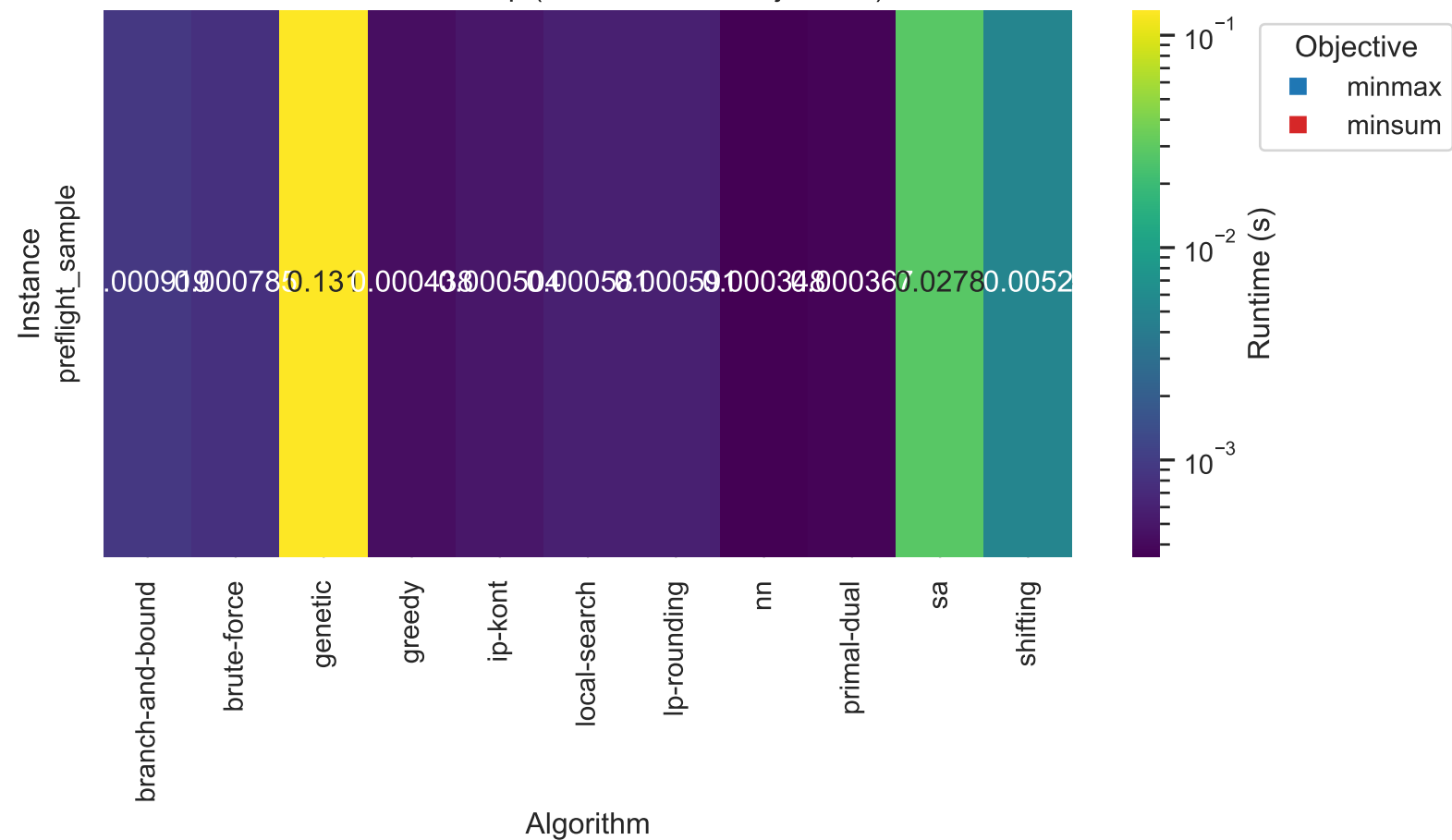
Runtime heatmap (median across objectives)
