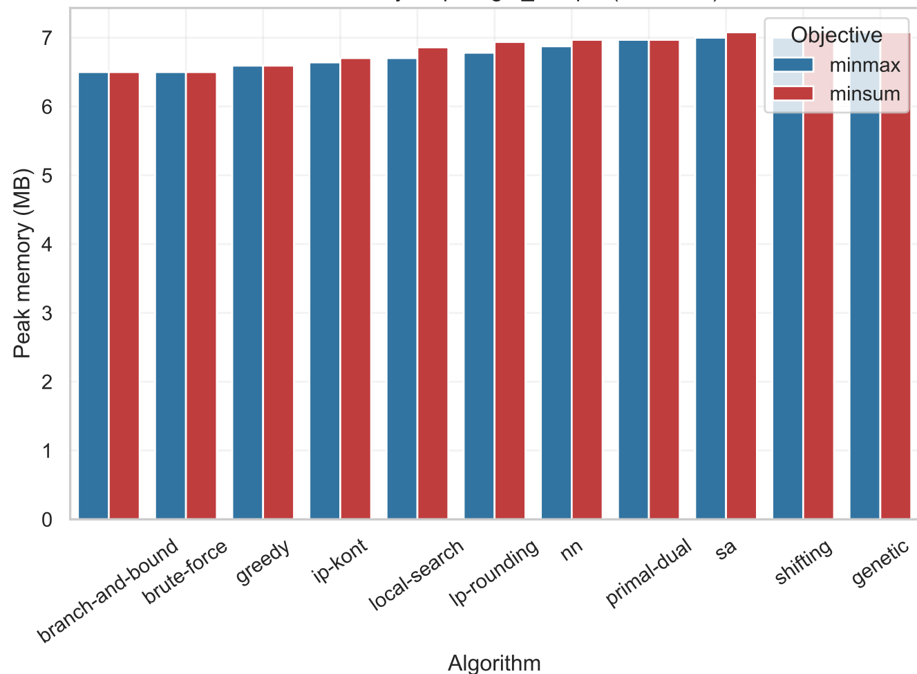
Peak memory on preflight_sample (n=2, m=2)
