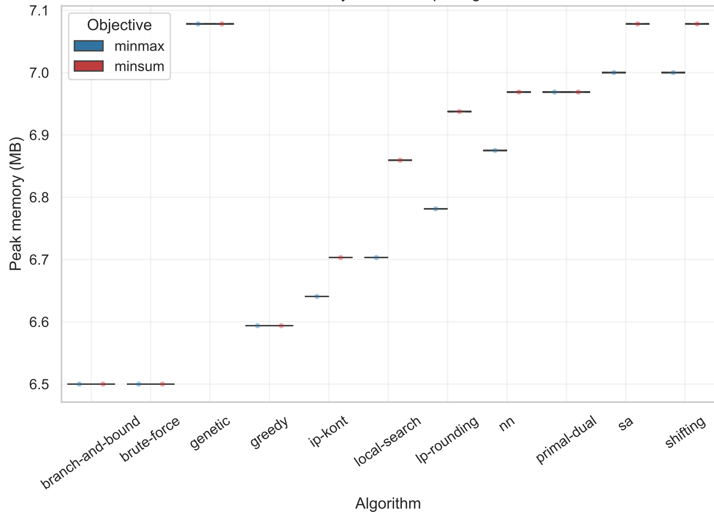
Peak memory distribution per algorithm
