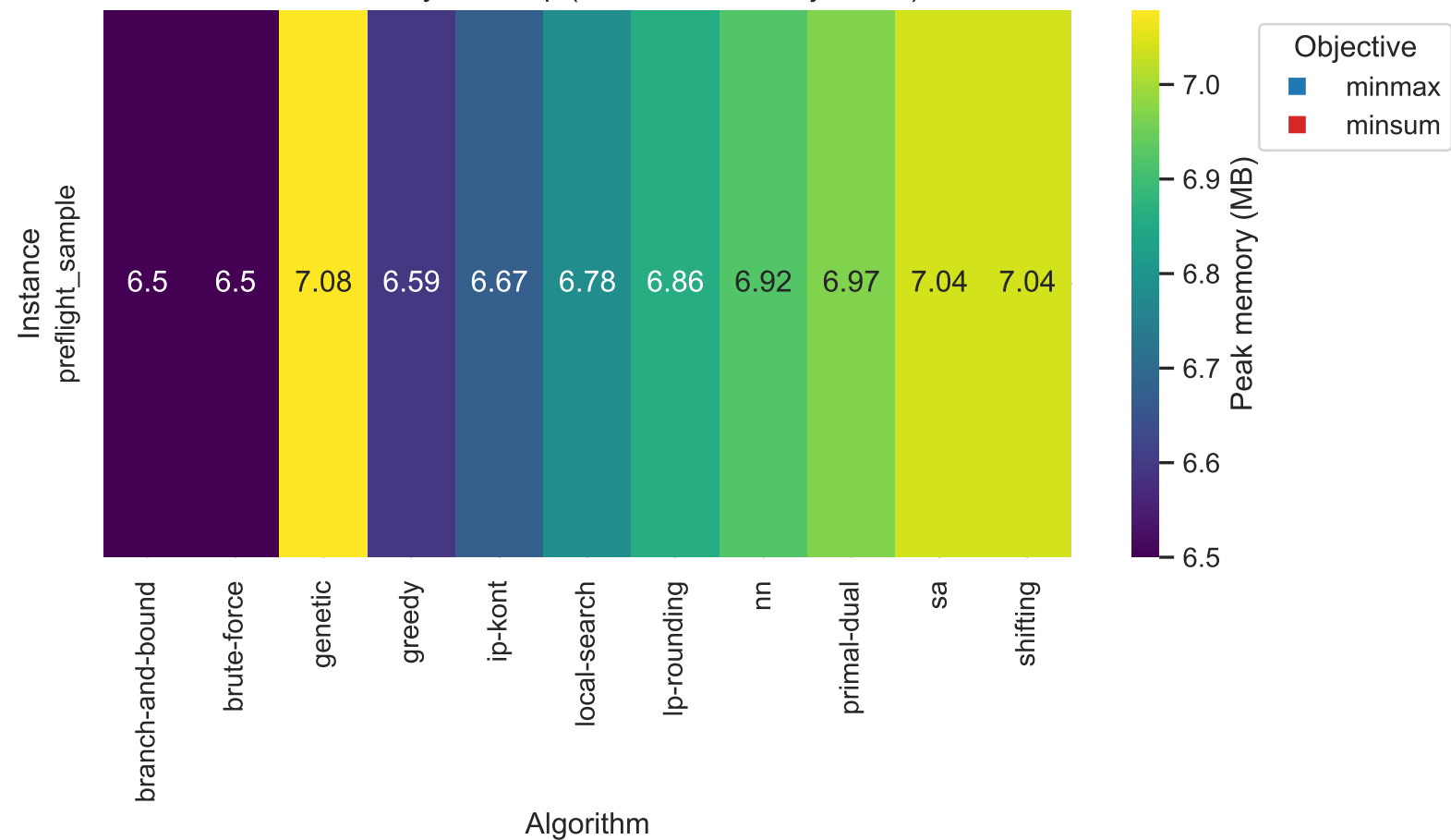
Peak memory heatmap (median across objectives)
