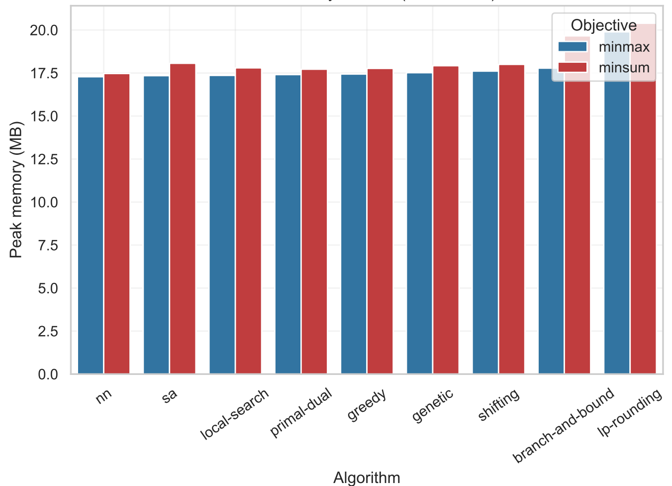
Peak memory on eil51 (n=13, m=25)
