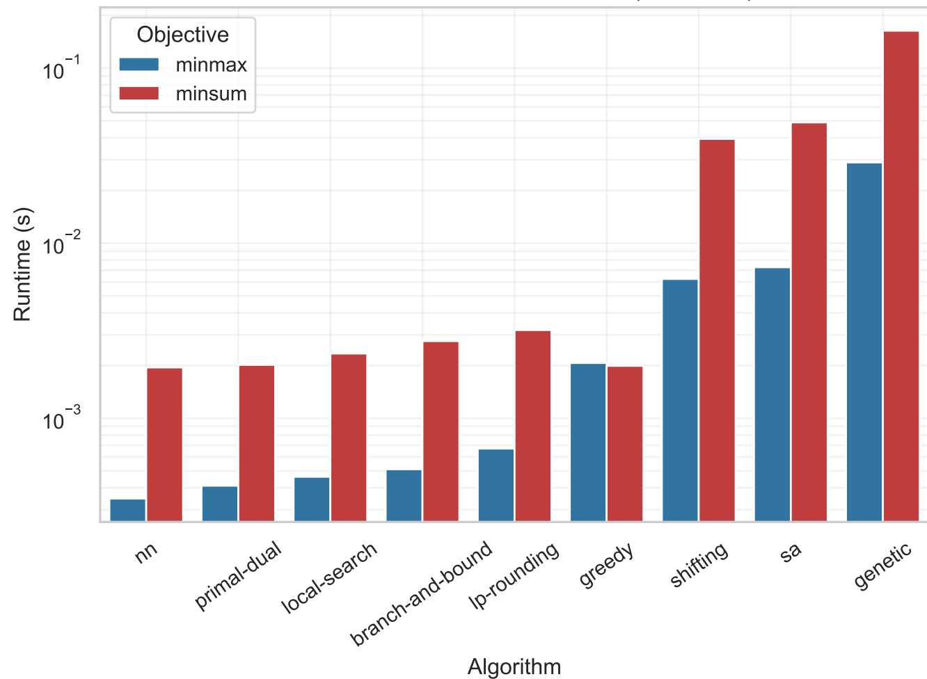
Runtime on stars-0000030.instance (n=2, m=25)
