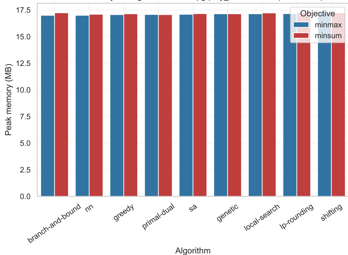
Peak memory on sbgdb-20200507-fpg-poly_0000000030 (n=1, m=25)
