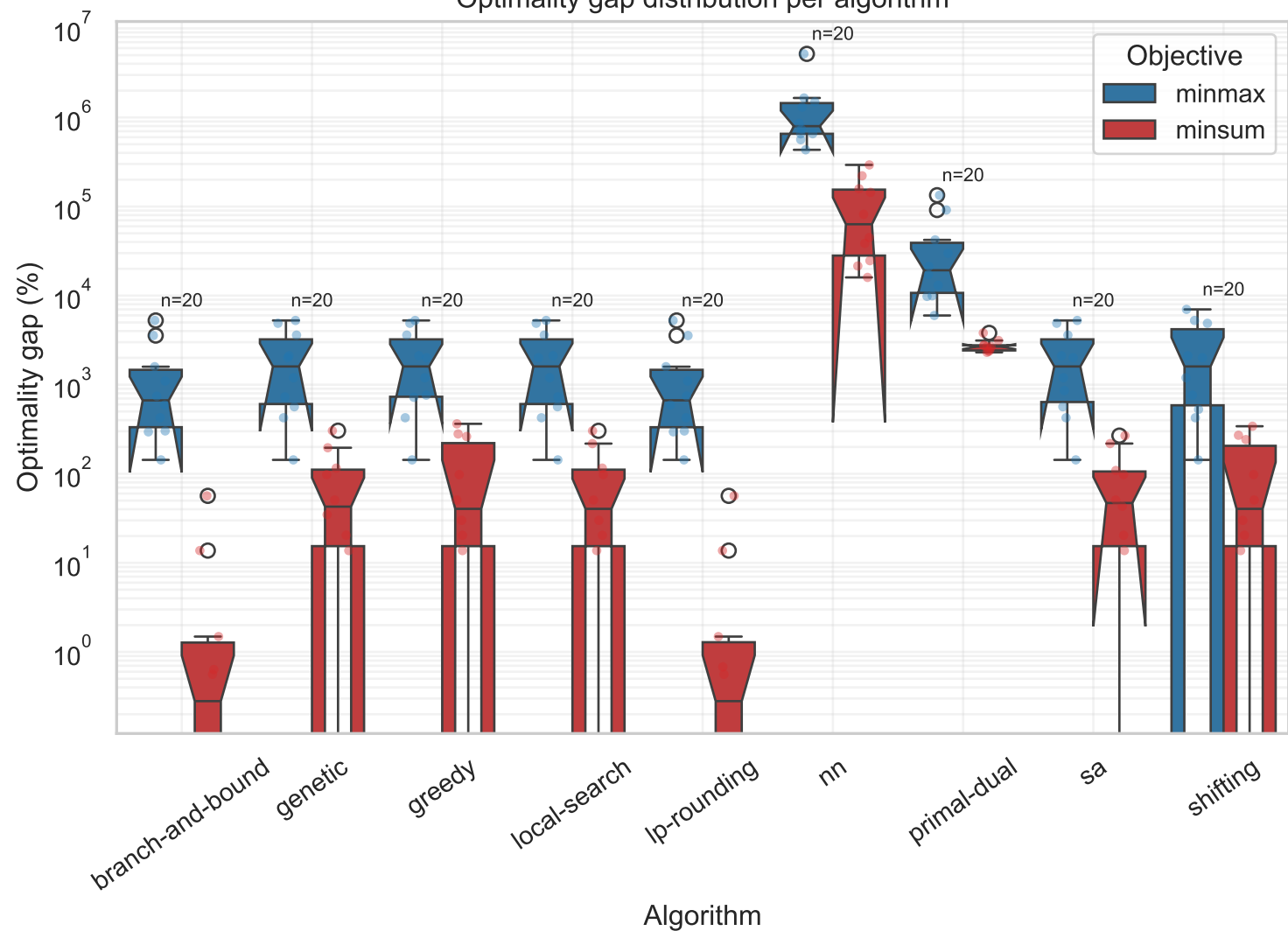
Optimality gap distribution per algorithm
