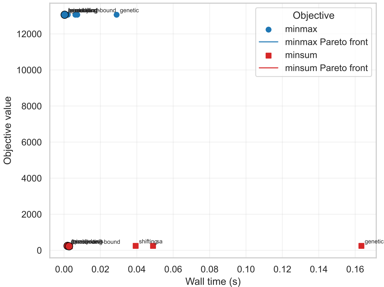
Pareto front on stars-0000030.instance
