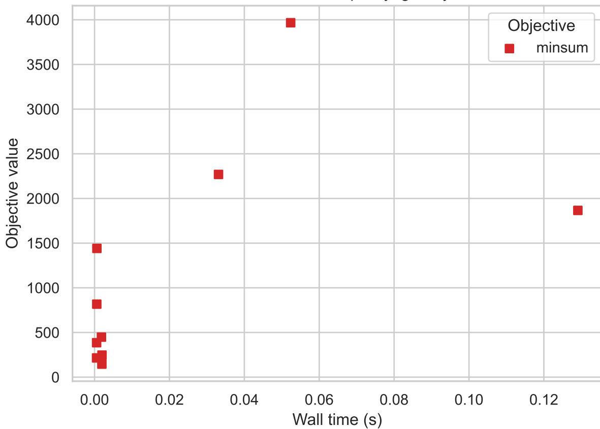
minsum runtime-quality: greedy
