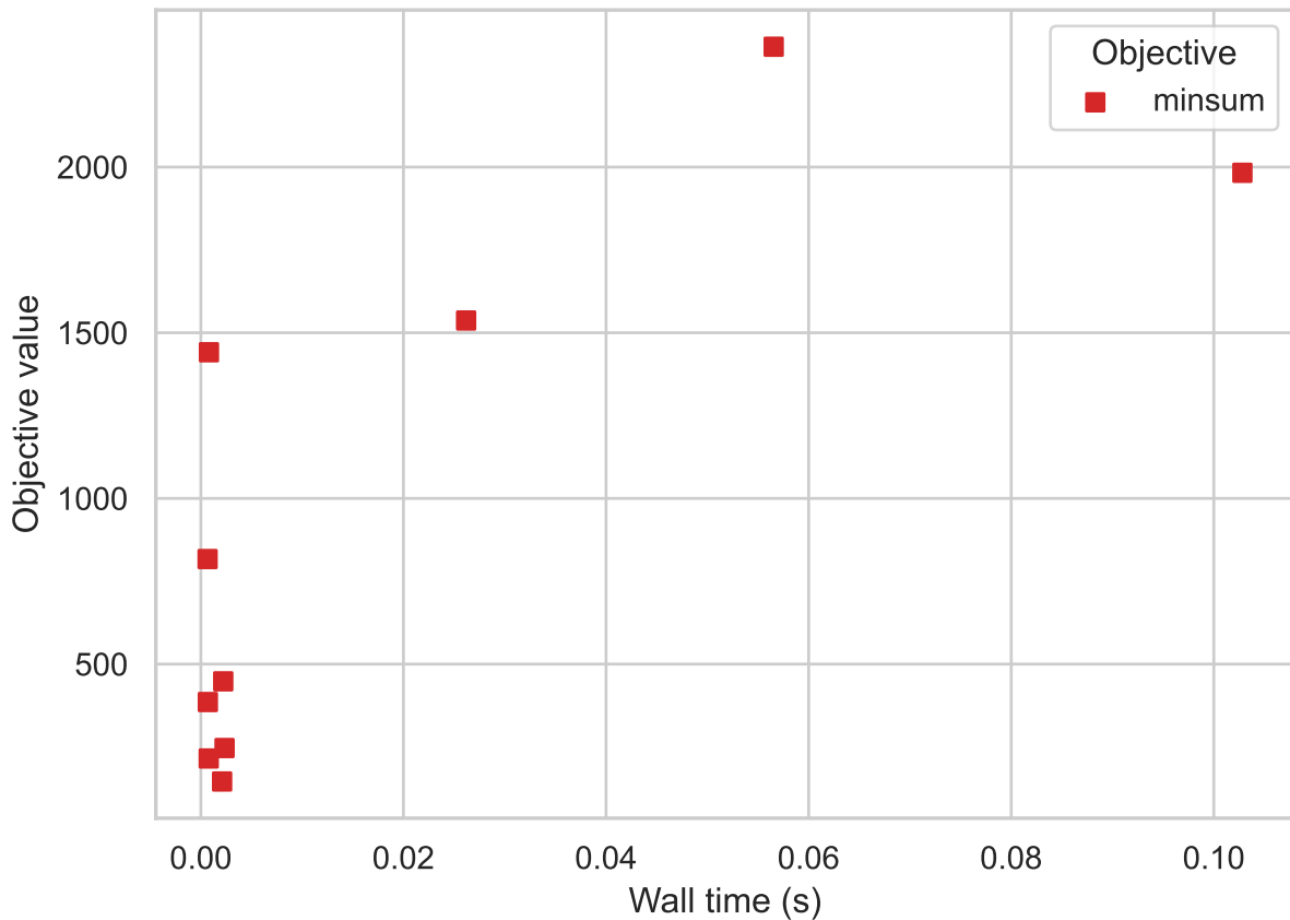
minsum runtime-quality: local-search
