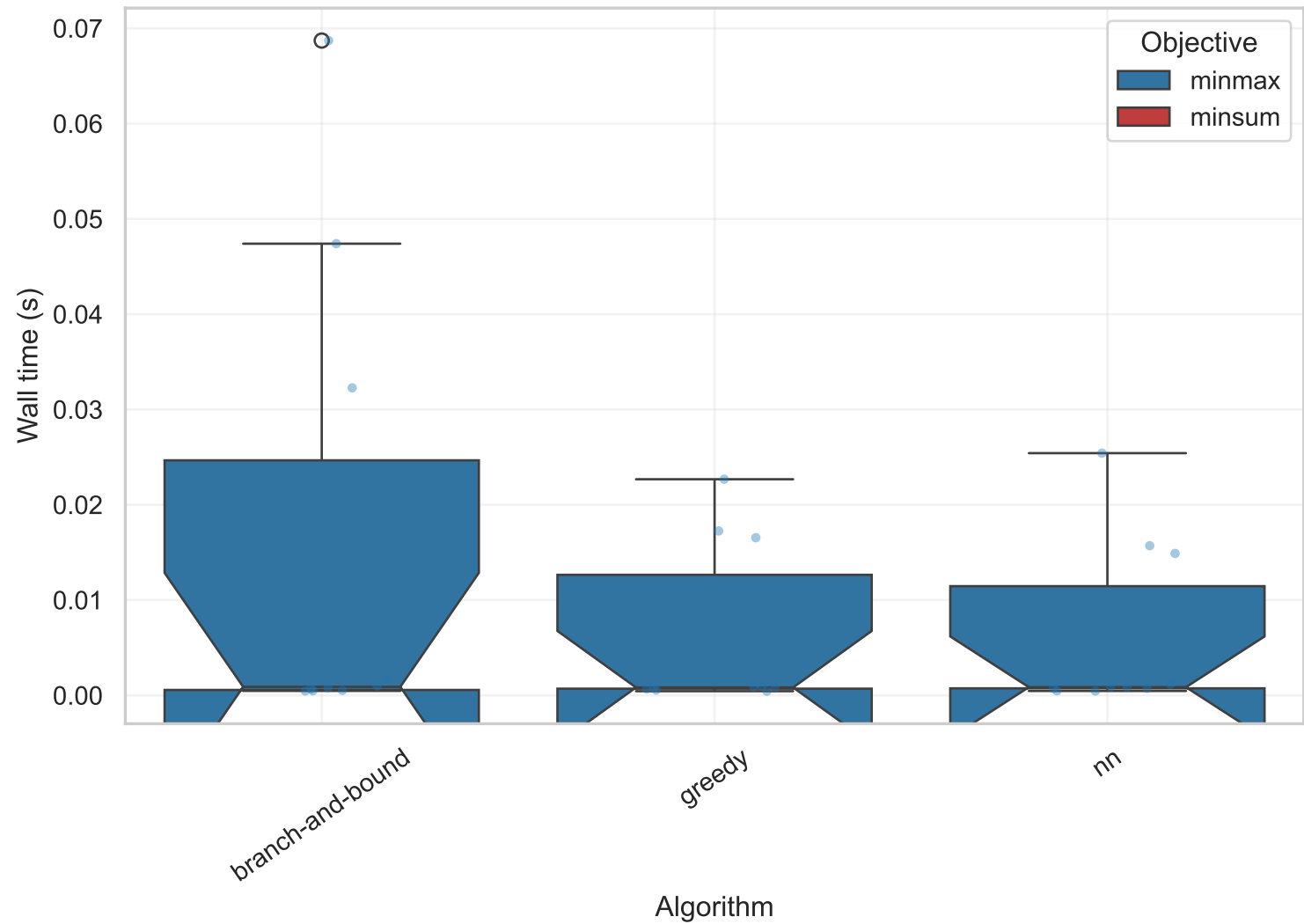
Runtime distribution per algorithm
